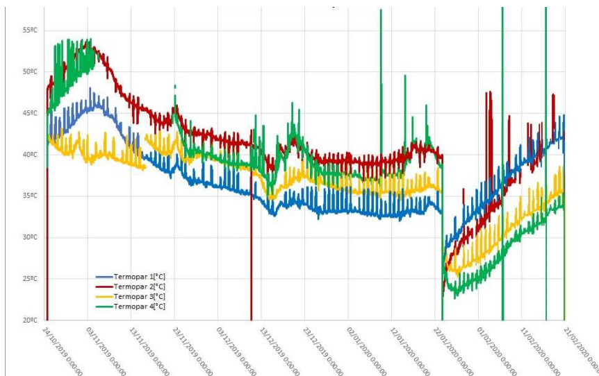
Figure 9 a, b, c: Changes in temperature detected by the thermocouples throughout the trial periods.
