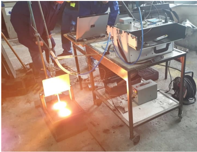
Small scale chamber tests at laboratory of AGH University in Poland
